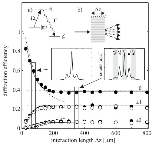
FIG. 1: Formation of a nonspeading Michelangelo wave packet for the center-of-mass motion of an open two-level atom (a). The resonant interaction with a standing light wave (b) leads to an array of harmonic imaginary potentials. The normalized diffraction efficiencies derived from the momentum distributions (inset) approach a steady state as a function of the interaction length \Delta z demonstrating the successful realization of stationary wave packets. The solid curves result from a numerical integration of the Schrödinger equation [16] with the Rabi frequency \Omega_0 = 0.4\Gamma . The dashed lines correspond to the Raman-Nath approximation, revealing that the interplay between absorption and quantum spreading is essential for obtaining a steady state.
