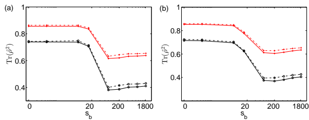
FIG. 5. Exact results (solid lines) and estimates (dashed lines) for the purity of system A ( \text{Tr}\hat{\rho}_A^2 , red lines with crosses) and of the combined bipartite system C ( \text{Tr}\hat{\rho}_C^2 , black lines with circles) for different strengths of the barrier for the ramping speeds (from left to right) 15.6 Hz/ms and 17.2 Hz/ms. The dashed lines show the estimates derived from our approximate expression of the density matrix based on direct experimental observables (5). Initial temperature T = 4\text{nK} . The relative sampling errors for the exact results are smaller than those shown in figure 2.
