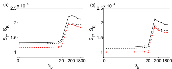
FIG. 3. Exact results for the total entropy S_T (solid lines) and its estimates (dashed lines) for different strengths of the barrier. The dashed black lines with crosses show the estimate derived from our approximate expression of the density matrix based on direct experimental observables (5); the red lines with circles show the estimate S_R from equation (A20) based on the Rényi entropies. Initial temperature T = 4\text{nK} for the ramping speeds (from left to right) 15.6 Hz/ms and 17.2 Hz/ms.
