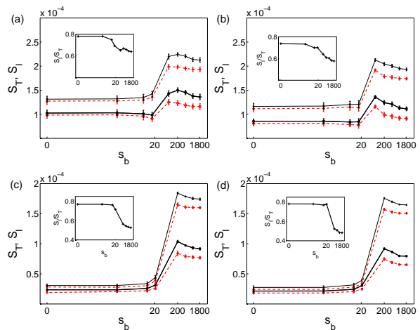
FIG. 2. Estimates (dashed lines) derived from (5) and exact results (solid lines) for the total entropy per atom S_T (lines with crosses) and internal entropy per atom S_I (lines with circles) for different strengths of the scissors. Top row: Initial temperature T = 4\text{nK} for the ramping speeds (from left to right) 15.6 Hz/ms and 17.2 Hz/ms. Bottom row: The same for T = 0 . The curve for the total entropy per atom is shown together with the sampling error calculated numerically over 800 individual stochastic realizations (see ). The insets show the ratio S_I/S_T (exact results) for each case.
