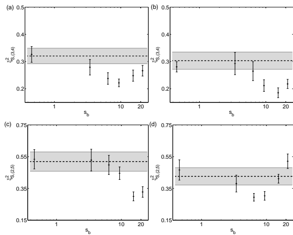
FIG. 4. Top row: Spin squeezing \xi_S^2 between the atoms in the two central lattice sites (sites 3 and 4 in figure 1) for different strengths of the scissors potential, with the ramping speeds (from left to right) 15.6 Hz/ms and 17.2 Hz/ms. Bottom row: Spin squeezing between the atoms in non-nearest-neighbour sites (sites 2 and 5 in figure 1), with the ramping speeds (from left to right) 15.6 Hz/ms and 17.2 Hz/ms. The dashed line shows the value obtained with no laser beam potential and the grey shaded area represents its uncertainty. The lattice is slowly ramped up to 72E_R after the barriers are rapidly introduced in thermal equilibrium at the lattice height 24E_R and T = 4\text{nK} .
