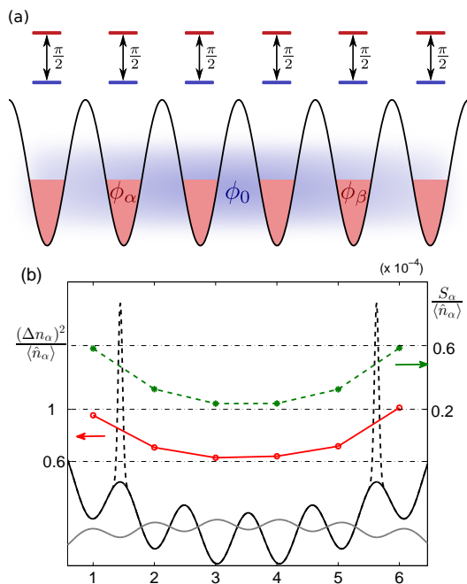
FIG. 1. (a) A schematic illustration of the relative phase measurement scheme. (b) Entropy engineering in the optical lattice where the tunneling of the atoms from the outermost sites to the rest of the system is suppressed, e.g., by applying symmetrically-positioned, tightly-focused, blue-detuned laser beams. We show the combined lattice potential and the optical barriers (black solid and dashed lines), the initial atom density before the sites are decoupled (solid grey line), the single-particle entropy S_\alpha / \langle \hat{n}_\alpha \rangle per atom in site \alpha (green dashed line with stars), and the normalized on-site atom number fluctuations (\Delta n_\alpha)^2 / \langle \hat{n}_\alpha \rangle (red solid line with circles) in the initial state for each lattice site. The temperature is assumed to be 4 nK.
