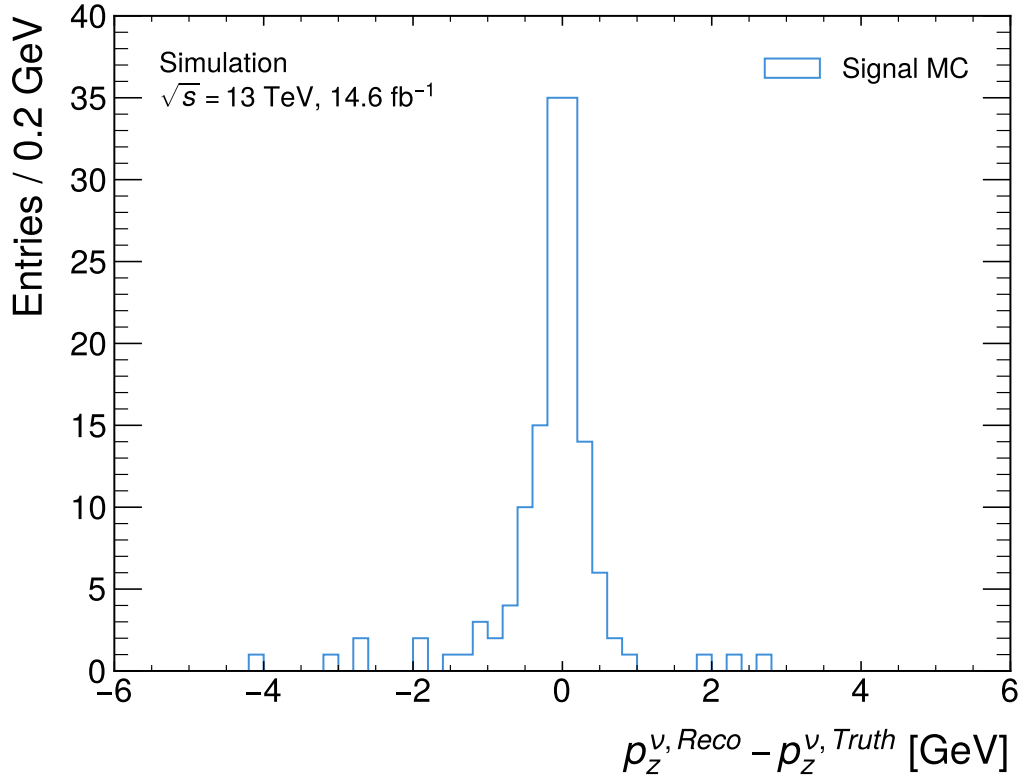
Figure A.1. Resolution of the neutrino p_z values for the signal process in the signal region. The reconstructed values are derived from the methodology discussed in this thesis and then compared to truth level information. The distribution demonstrates that the value is well modelled.
