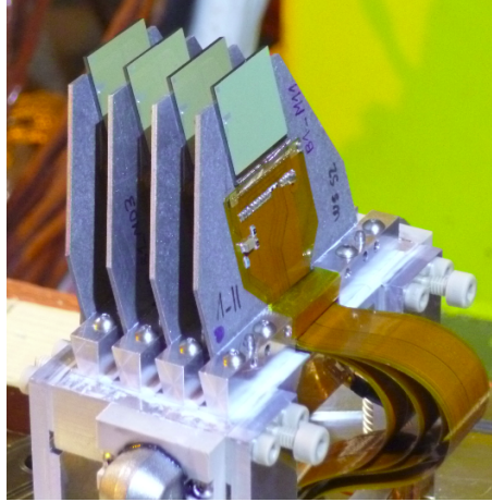
Figure 3.7. Photo of AFP SiT of a station. Pixel trackers are located on a heat exchange. Taken from Ref. [71].
