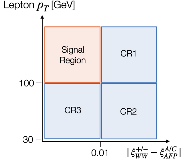
Figure 7.11. Signal region and control regions defined for the boosted channel. Regions are defined in the kinematic plane of leading lepton p_T and |\xi_{WW}^{\pm/-} - \xi_{AFP}^{A/C}| .
