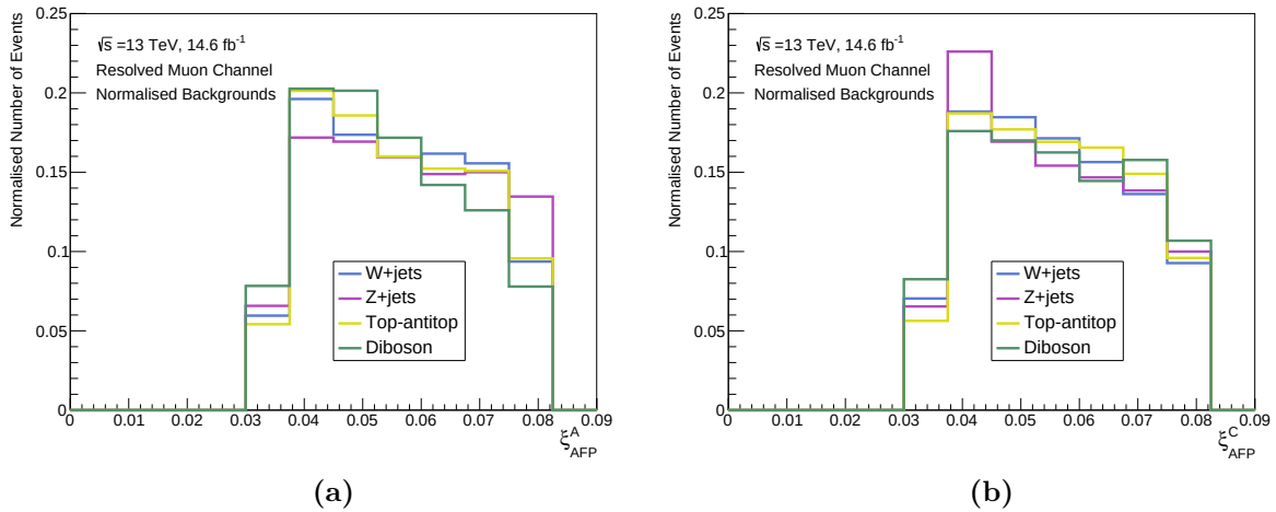
Figure D.1. Normalised \xi_{\text{AFP}}^{\text{A/C}} distributions of simulated background processes in the inclusive region where background estimation is determined. Shown are the distributions for the resolved muon channel on the A side (Fig.D.1a) and C side (Fig.D.1b).
