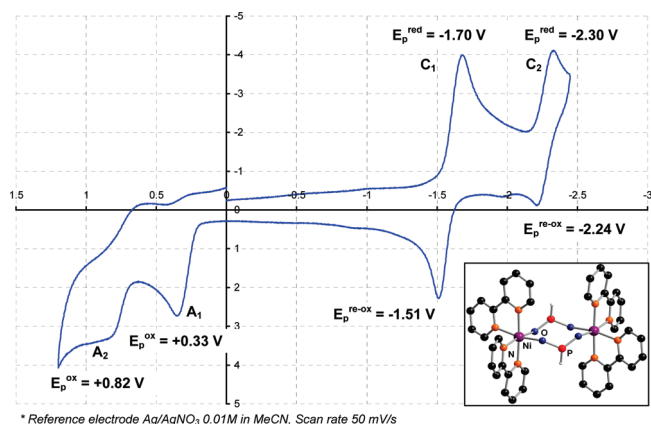
Figure 3. Cyclic voltammogram of 3a in DMF (room temperature).
