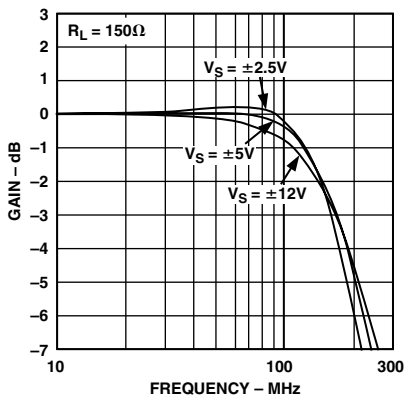
TPC 25. AD8129 Frequency Response vs. Supply, R_L = 150\ \Omega
