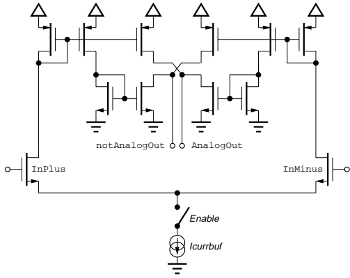
Figure 8: Schematic of the fully differential current driver on Beetle 1.3.
