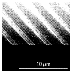
SEM image of one of the silicon grating of TGZ Series.
