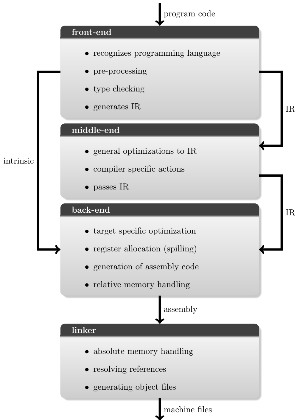
Figure 1.1: Schematic Compiler Structure
