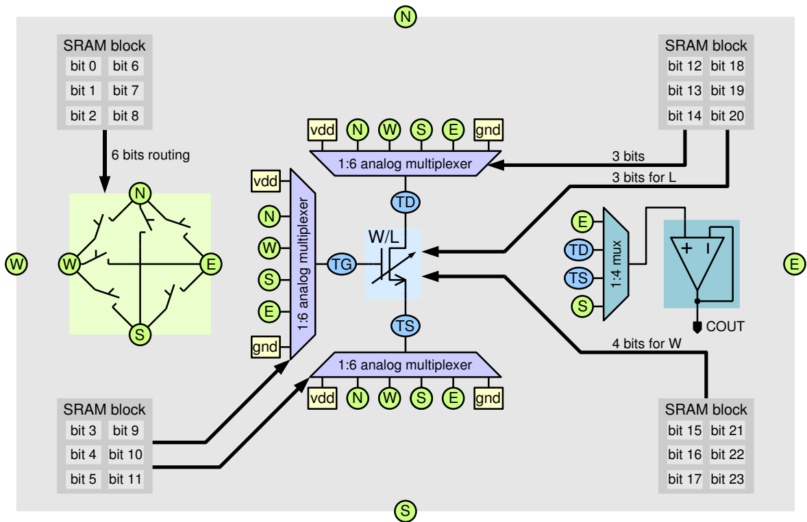
Figure 3.2: Simplified architecture of the complete NMOS transistor cell. The correct assignment of configuration bits is documented in Table 3.1 and Table A.1.
